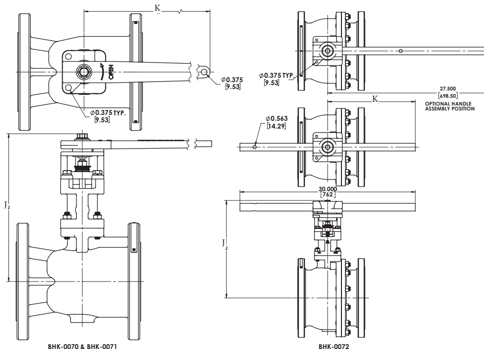
Series 7150 Emission-Pak ASME Class 150 Approximate Dimensions - inches
